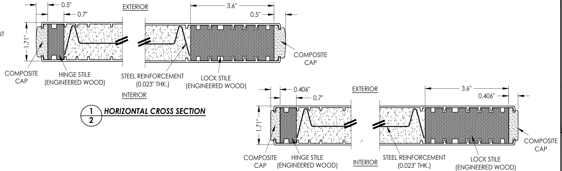
2 HORIZONTAL CROSS SECTION
